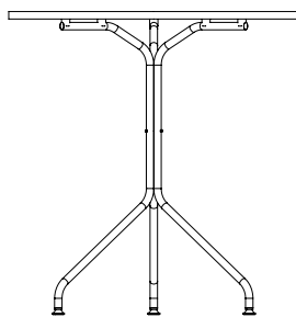
STOLEK
